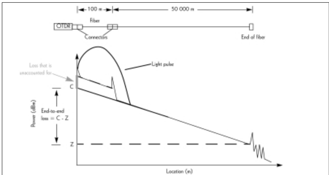
Figure 2. OTDR loss measurement with a 100 m pluse
